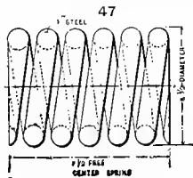
Fig. 1401. Center-spring.
